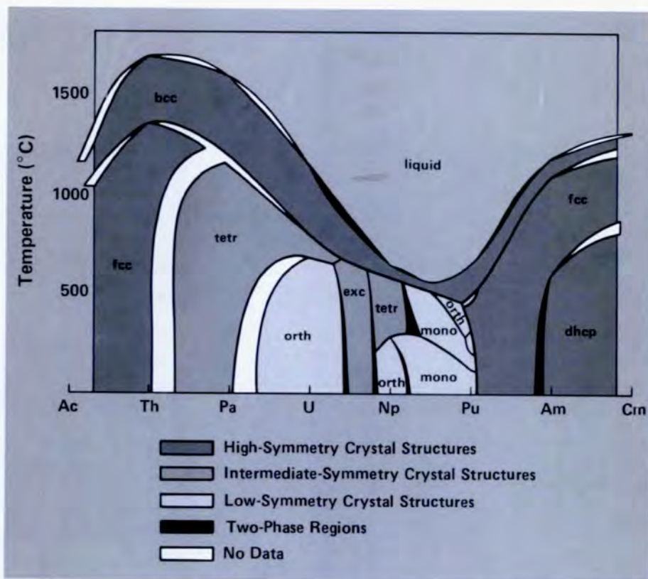
Fig. 2. A connected phase diagram of binary alloys of the actinides (prepared by E. A. Kmetko and J. L. Smith) shows the preponderance of low-symmetry crystal structures, the large number of phase changes, and the depression of melting points in the vicinity of plutonium. The crystal structures are body-centered cubic (bcc), face-centered cubic (fcc), tetragonal (tetr), orthorhombic (orth), exotic cubic (exc), monoclinic (mono), and double hexagonal close-packed (dhcp).
